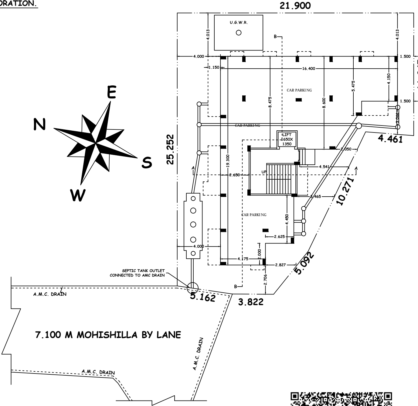
SEWAGE CONECTION PLAN SCALE 1:1
